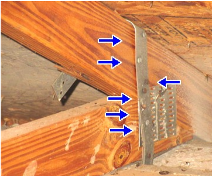
WALL TO ROOF CONNECTION
